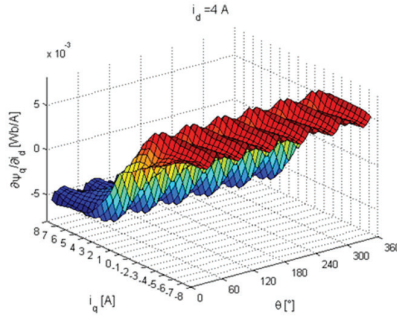
Figure 3: Graphic representation of the distribution of partial derivation \partial \Psi_q / \partial i_d for current i_d = 4 \text{ A}
